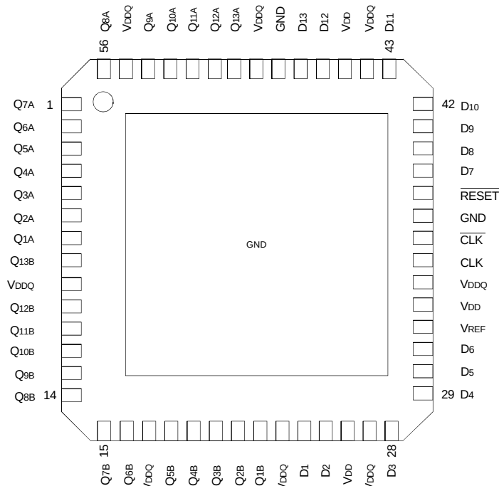
MLF TOP VIEW
