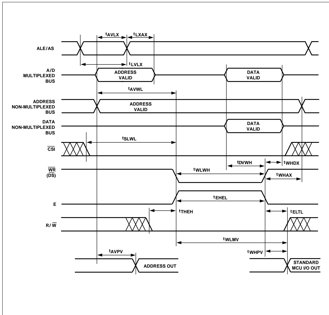
Figure 30. Write Timing
