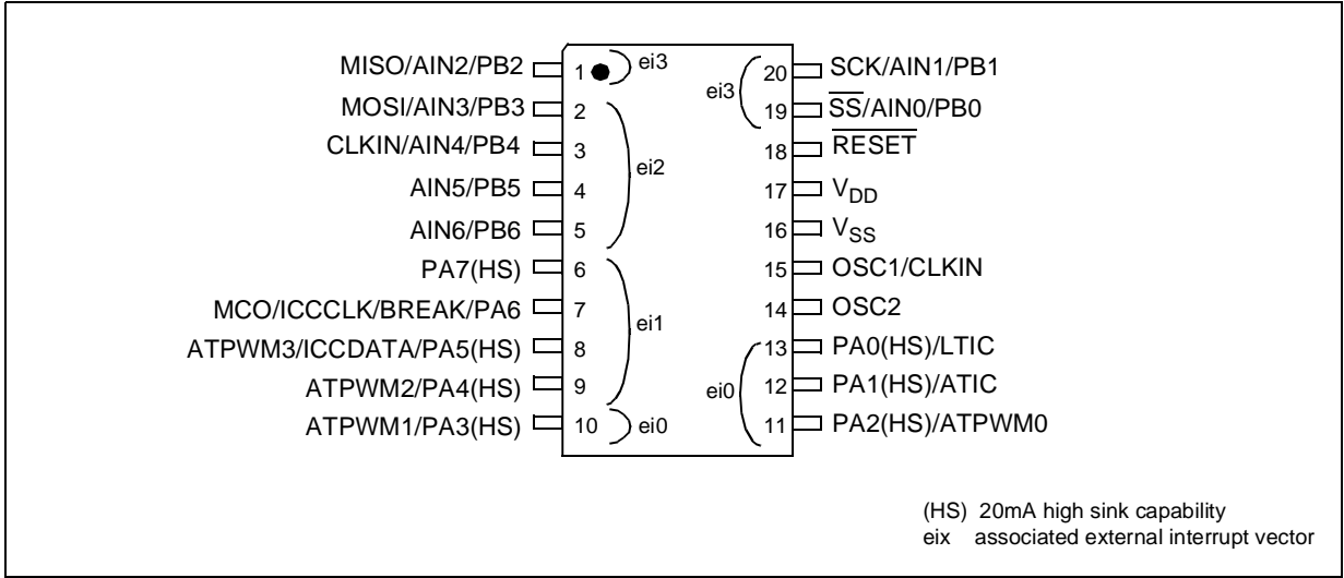
Figure 3. 20-Pin DIP Package Pinout (ST7LITE2x)
