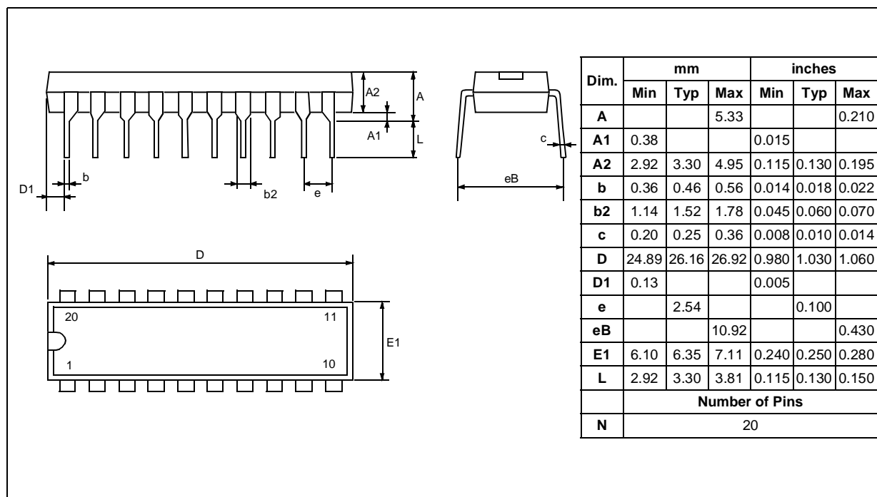
Figure 96. 20-Pin Plastic Dual In-Line Package, 300-mil Width
