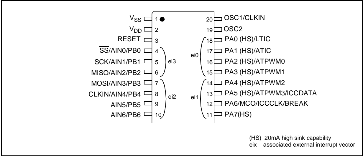
Figure 2. 20-Pin SO Package Pinout (ST7LITE2x)
