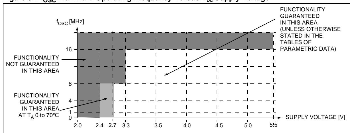
Figure 52. f_{OSC} Maximum Operating Frequency Versus V_{DD} Supply Voltage
