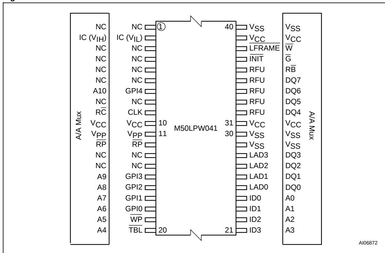
Figure 4. TSOP Connections
