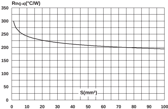
Fig. 9: Thermal resistance junction to ambient versus copper surface under each lead (epoxy printed board FR4, Cu=35μm, typical values).
