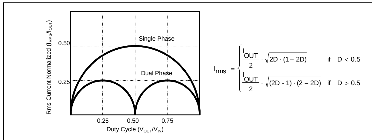
Figure 12. Input RMS Current vs. Duty Cycle (D) and Driving Relationships
