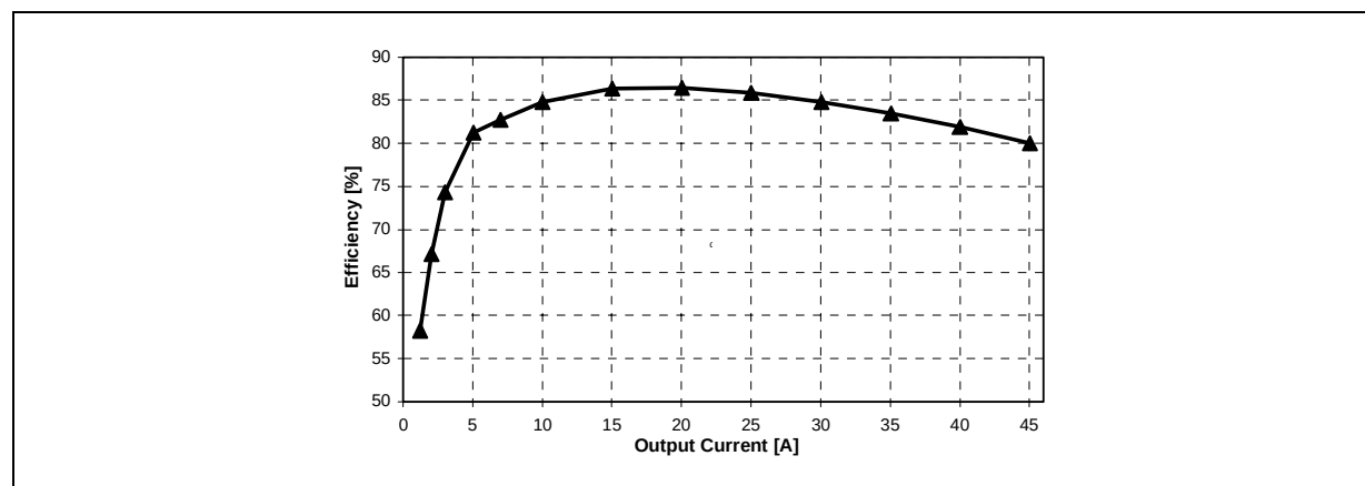
Figure 25. System Efficiency
