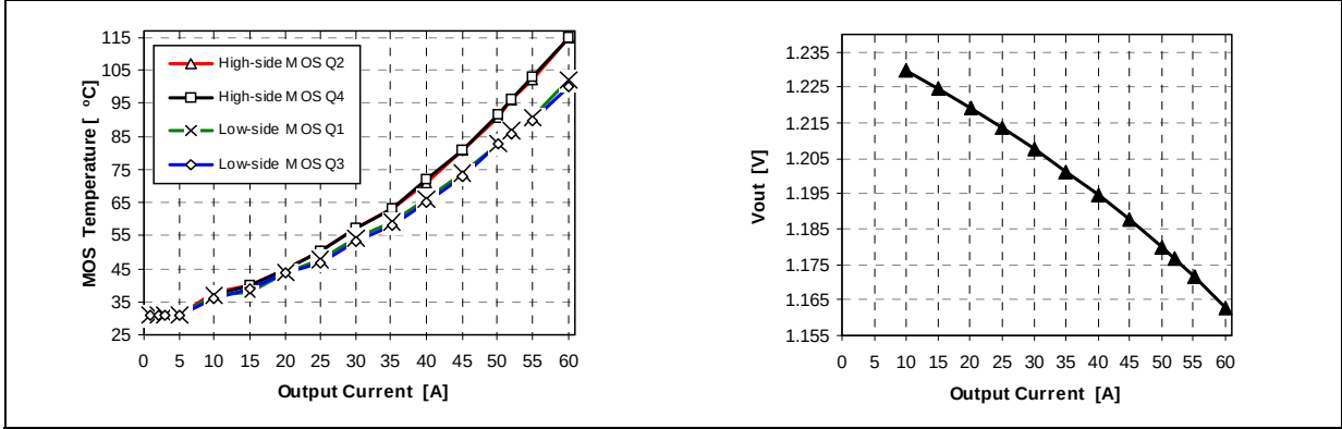
Figure 30. Mosfet Temperature and Load Regulation.
