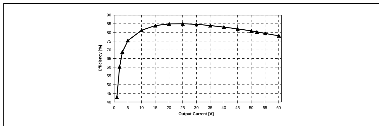
Figure 29. System Efficiency
