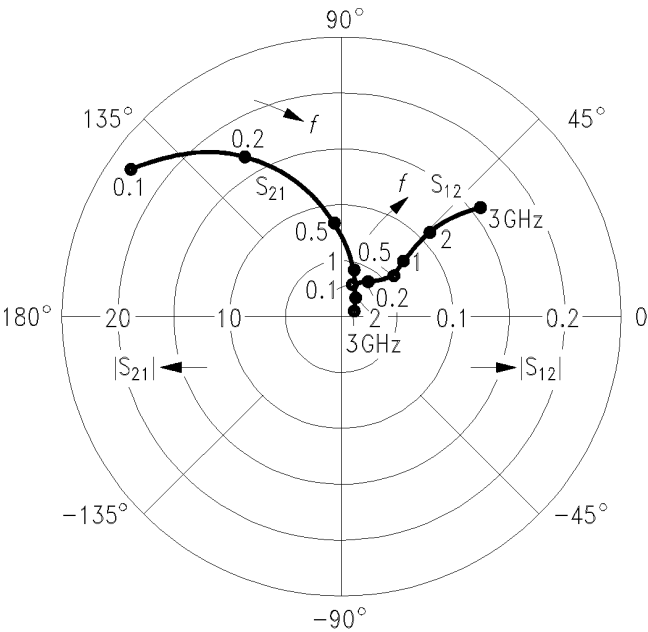
S 12 , S 21 = f ( f ) I C = 10 mA, V CE = 5 V, Z 0 = 50 Ω
