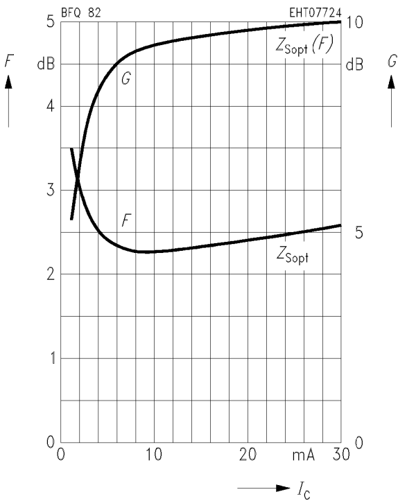
Noise figure F = f(I_c) Power gain G = f(I_c) V_{CE} = 8\text{ V} , f = 2\text{ GHz} , Z_{Lopt}(G)
