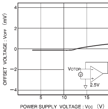
Fig. 7 Power supply voltage vs. I/O offset voltage
