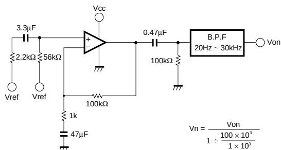
Fig. 8 Input conversion noise voltage
