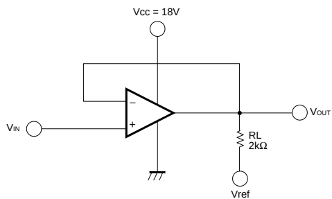
Fig. 5 Slew rate ( I )
