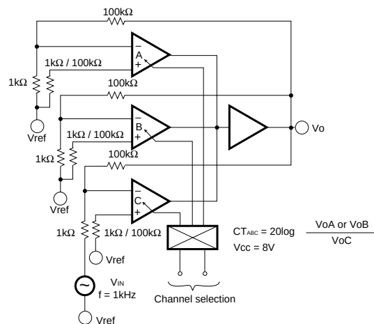
Fig. 9 Crosstalk between A and B
