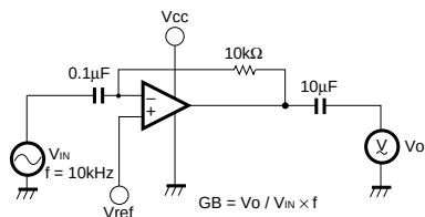
Fig. 7 Band width frequency gain
