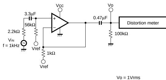
Fig. 10 Total harmonic distortion
