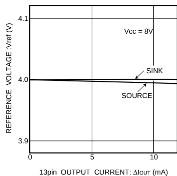
Fig. 17 Reference voltage vs. pin 13 output current
