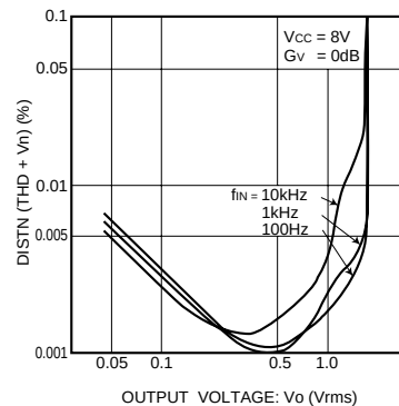
Fig. 16 Distortion vs. output voltage
