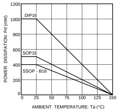
Fig. 4 Power dissipation vs. ambient temperature
