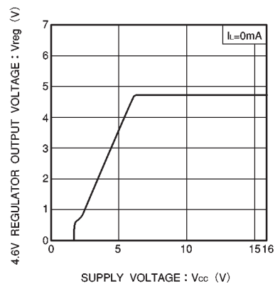
Fig.8 4.6V constant-voltage source output voltage characteristics
