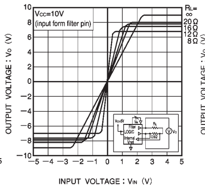
Fig.4 I / O characteristics with governor connected
