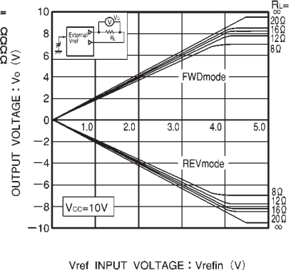
Fig.5 Reversible driver I / O characteristics
