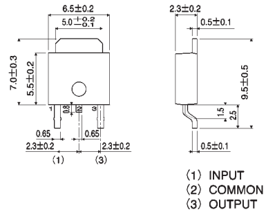
TO252-3
