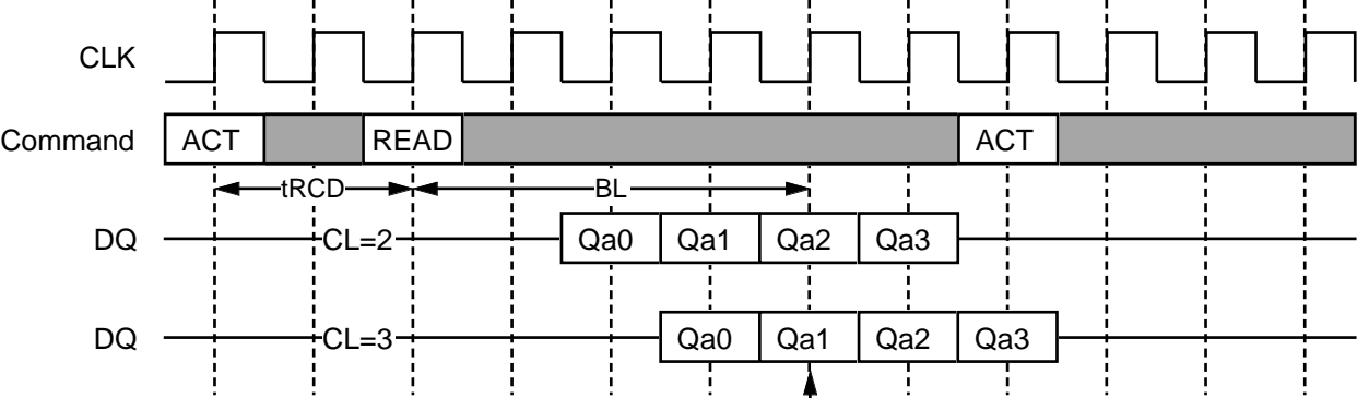
Auto-Precharge Timing (READ, BL=4)
