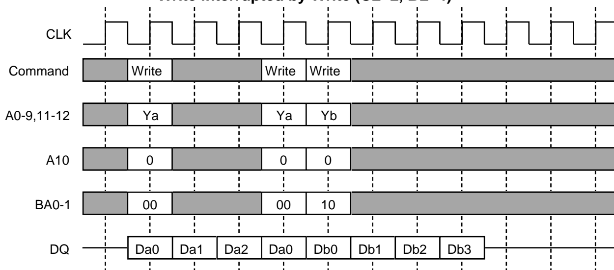
Write interrupted by Write (CL=2, BL=4)
