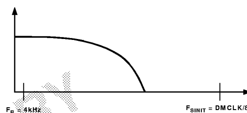
a. Analog Antialias Filter Transfer Function
