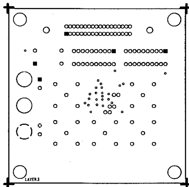
c. AD9850/CGPCB Power Plane
