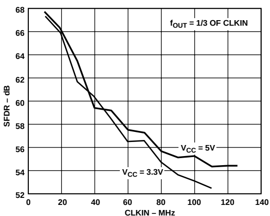
Figure 8. SFDR vs. CLKIN Frequency ( A_{OUT} = 1/3 of CLKIN)
