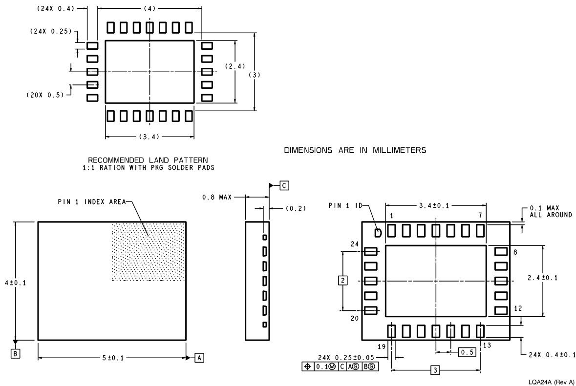
24-Lead Package LQA Order Number ADC1175-50CILQX NS Package Number LQA24A
