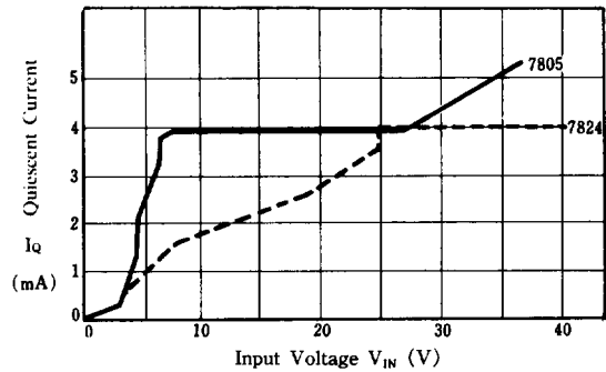
NJM7805/24 Quiescent Current vs. Input Voltage ( T_j = 25^\circ\text{C} )
