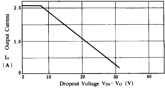
NJM7800 Series Short Circuit Output Current ( T_j = 25^\circ\text{C} , \infty Heat Sink)
