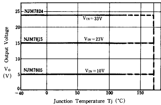
NJM7805/15/24 Output Voltage vs. Junction Temperature
