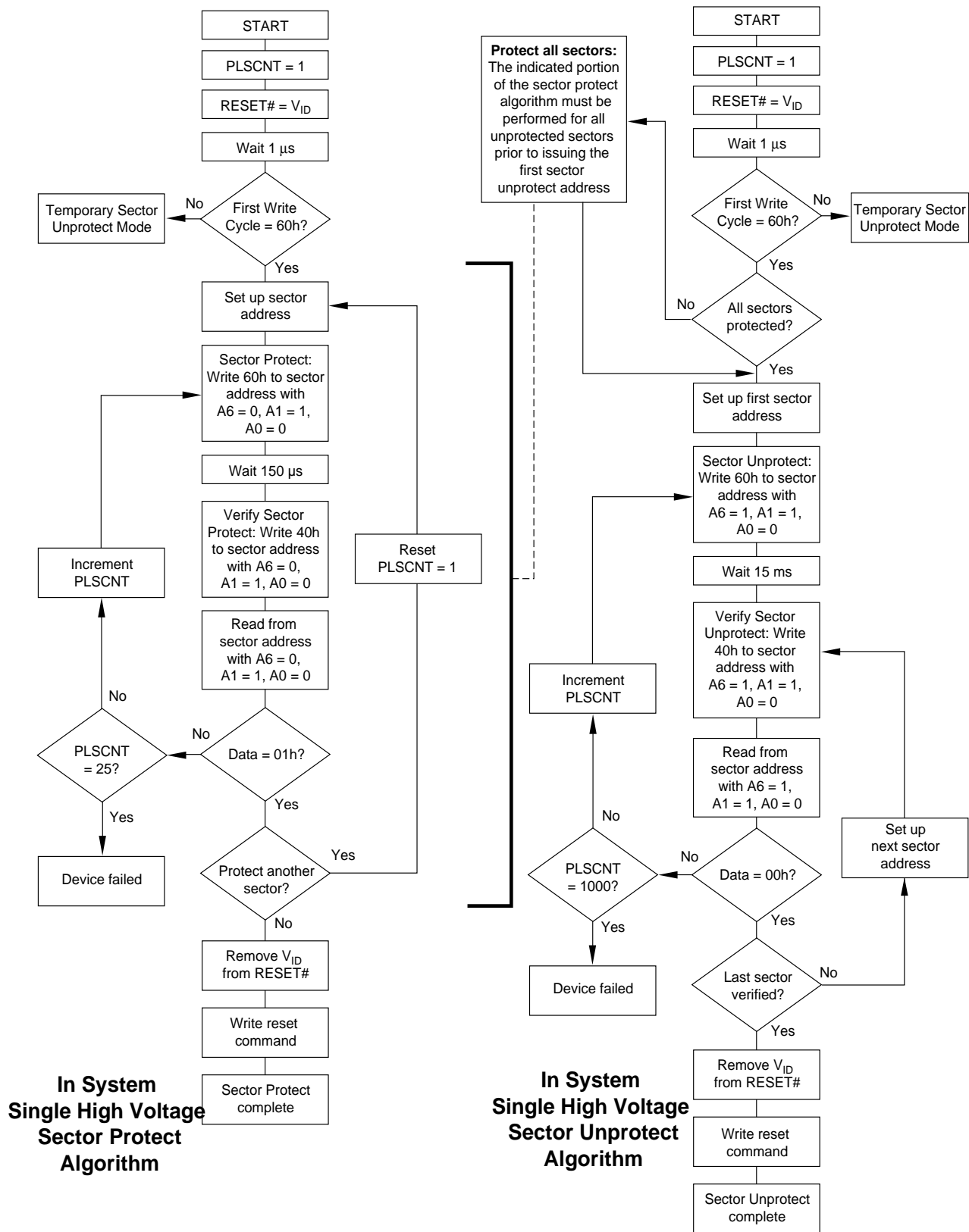
Figure 1. In-System Single High Voltage Sector Protect/Unprotect Algorithms
