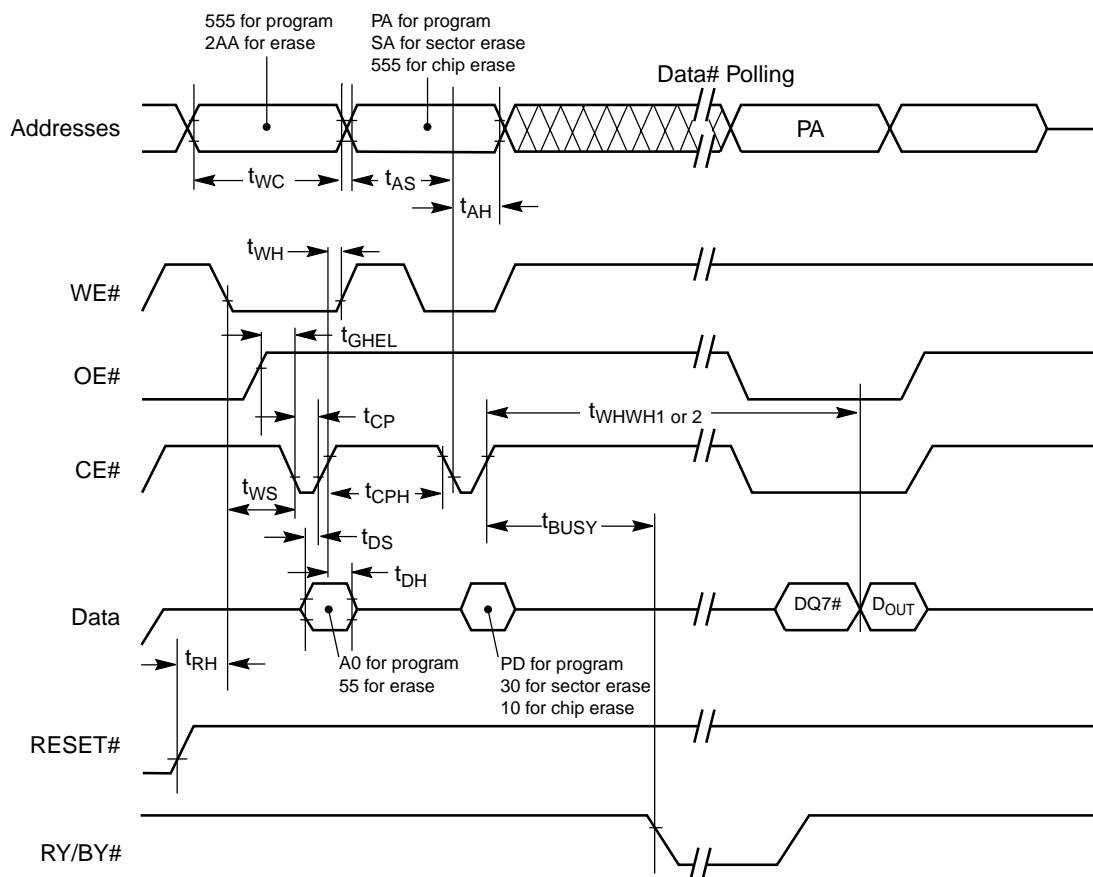
Figure 20. Alternate CE# Controlled Write Operation Timings
