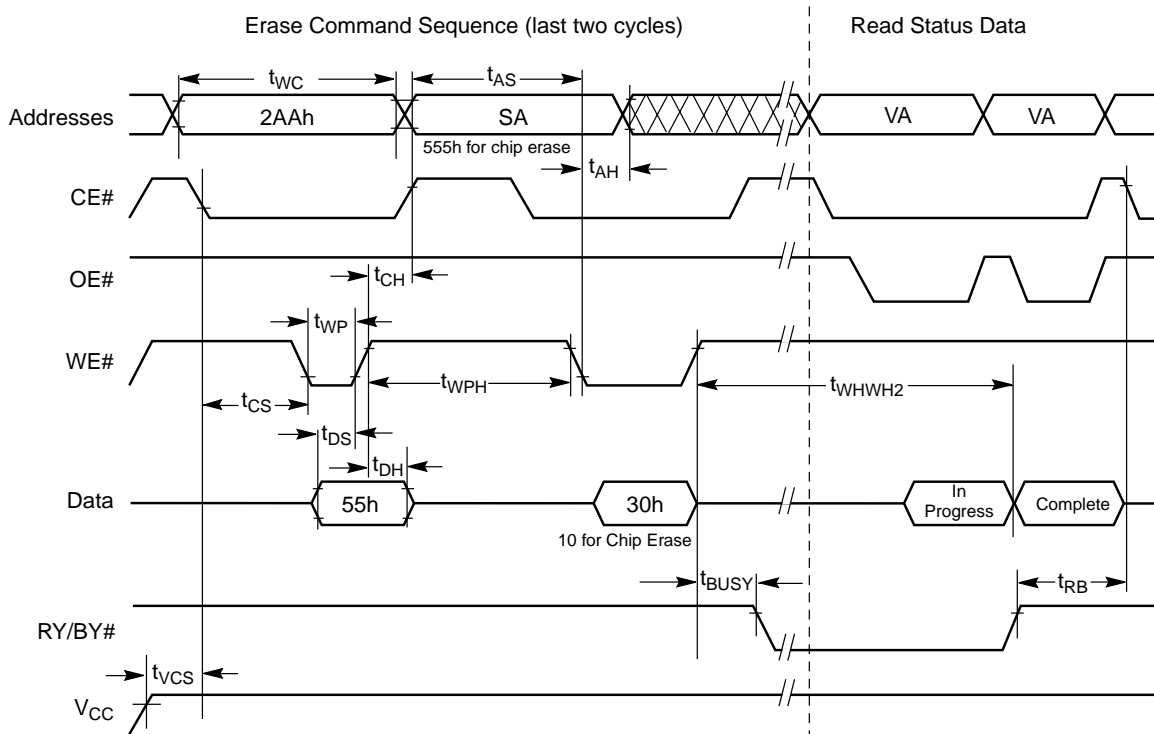
Figure 14. Chip/Sector Erase Operation Timings
