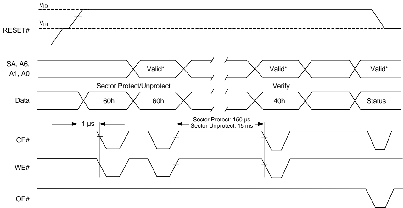
Figure 19. Sector Protect/Unprotect Timing Diagram
