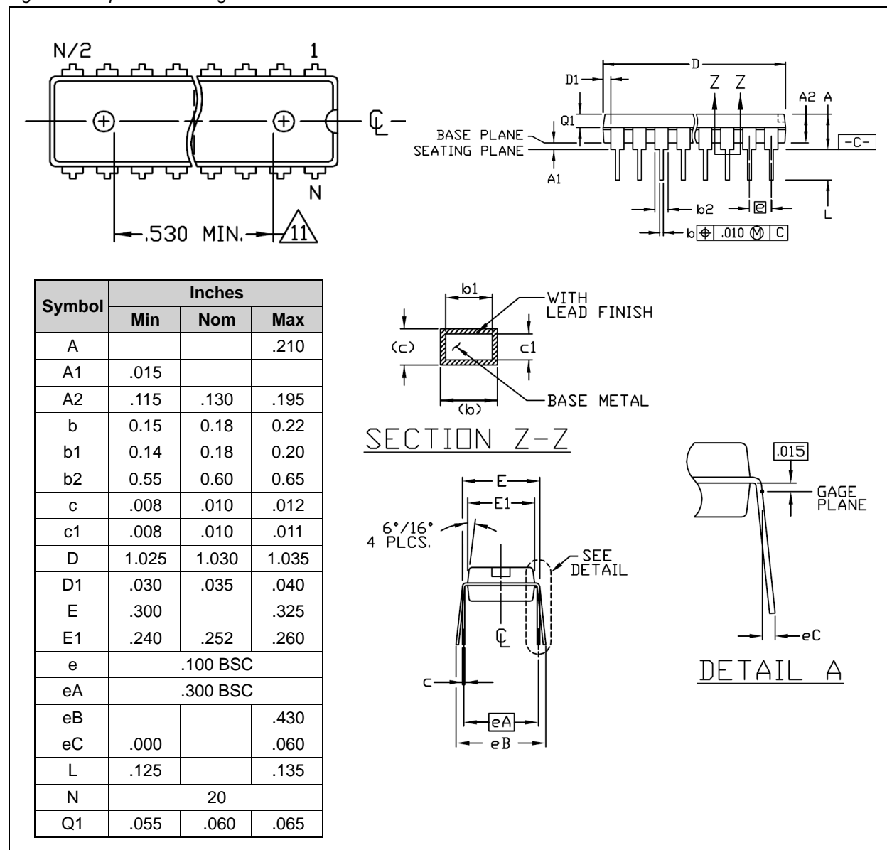
Figure 6. 20-pin DIP Package
