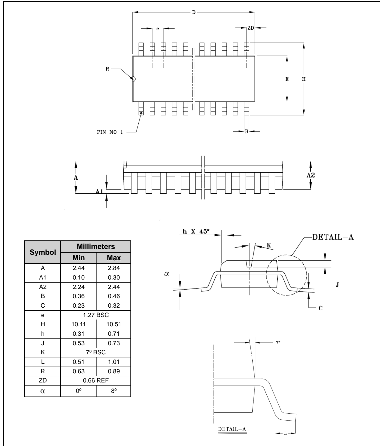
Figure 7. 20-pin SOIC Package
