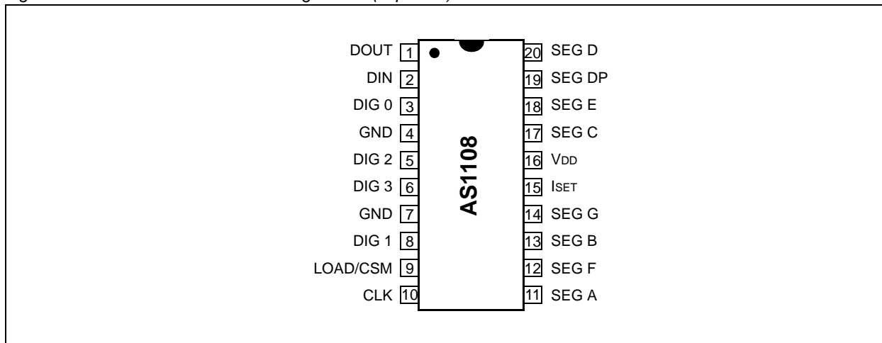
Figure 5. AS1108 DIP and SO Pin Assignments (Top View)
