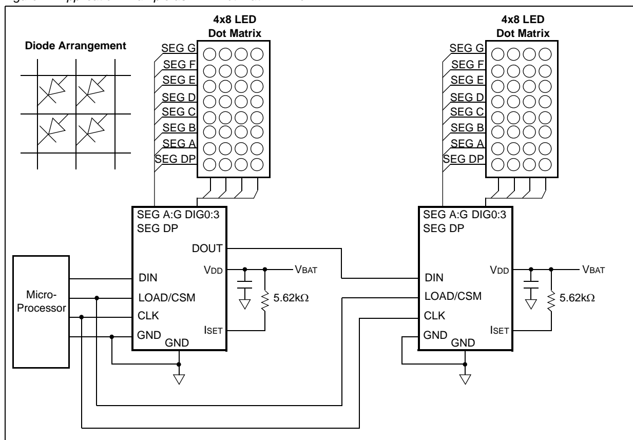
Figure 4. Application Example as LED Dot Matrix Driver
