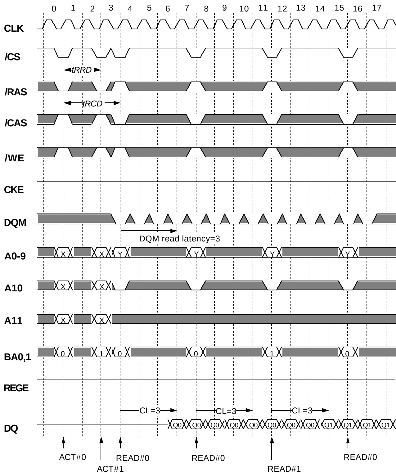
Page Mode Burst Read (multi bank)
