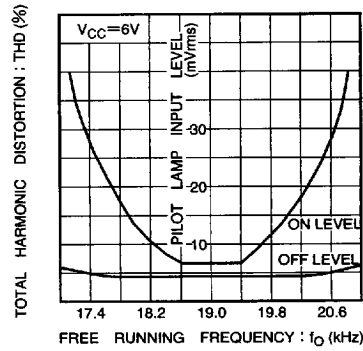
Fig. 7 Lamp on and off levels vs. free-running frequency
