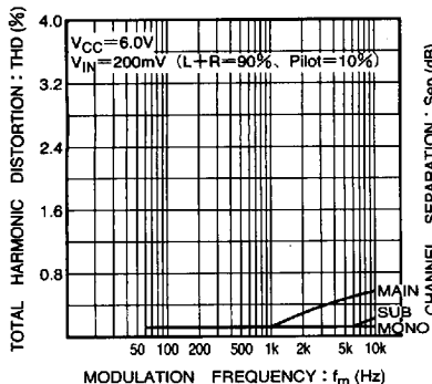
Fig. 2 Total harmonic distortion vs. modulation frequency
