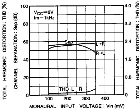
Fig. 6 Total harmonic distortion and channel separation vs. monaural input voltage
