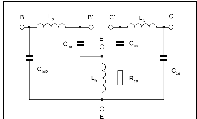
Fig.16 Package equivalent circuit SOT343R2.
