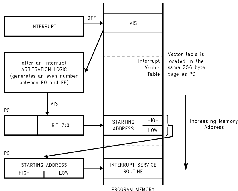
FIGURE 29. VIS Operation
