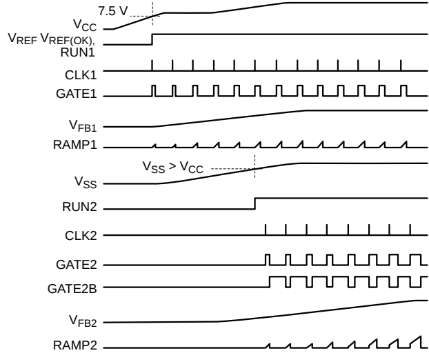
Figure 3. Startup Waveforms
