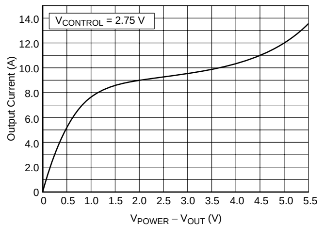
Figure 6. Short Circuit Current vs V POWER - V OUT
