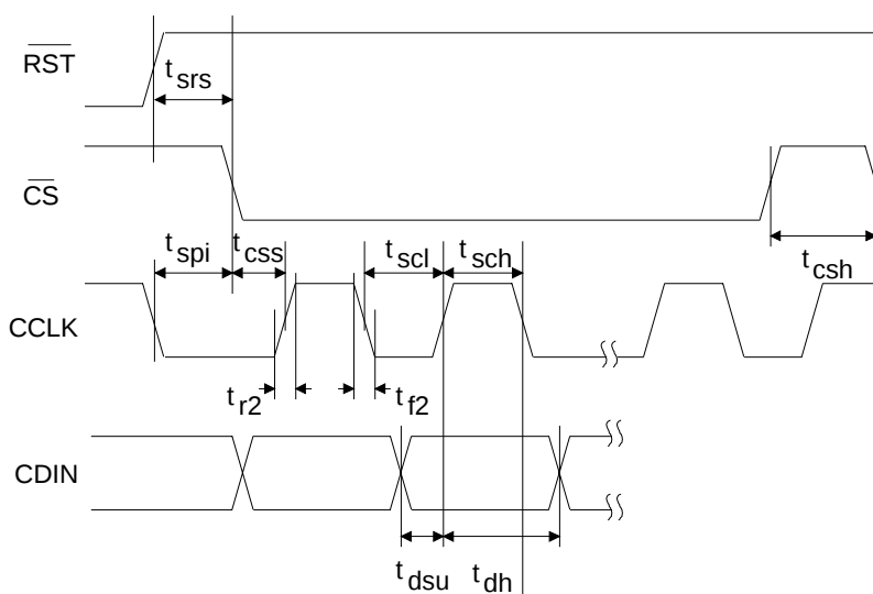
Figure 4. Control Port Timing - SPI Mode
