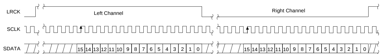
Figure 18. CS53L32A Control Port Mode - Serial Audio Format 1
