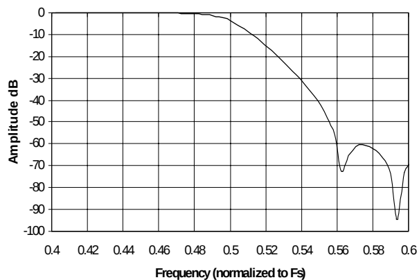
Figure 9. Base-Rate Transition Band
