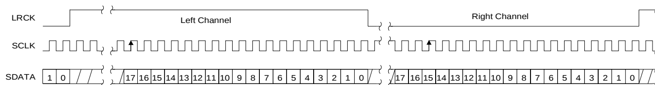
Figure 20. CS53L32A Control Port Mode - Serial Audio Format 4
