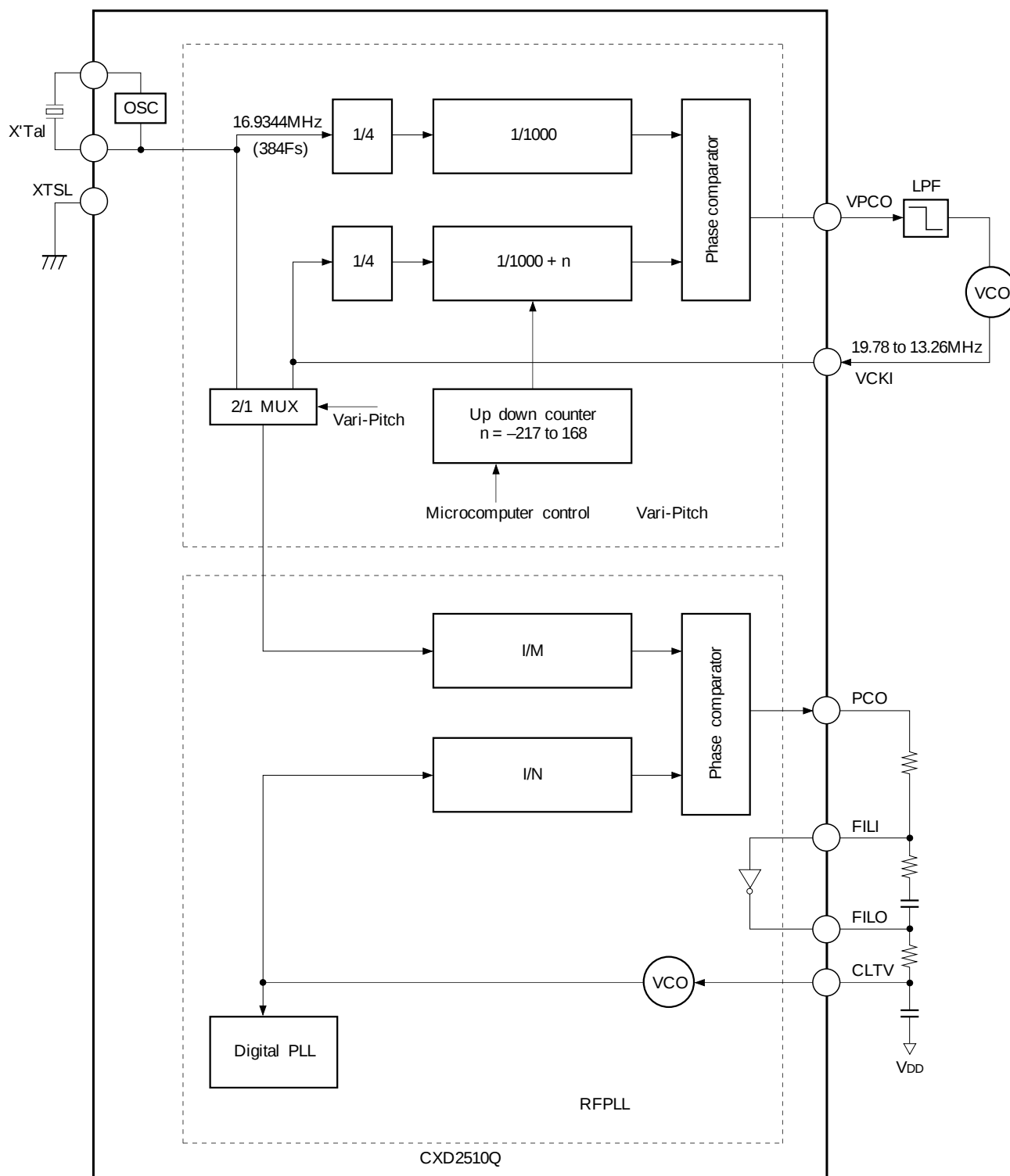
Block Diagram 3-1
