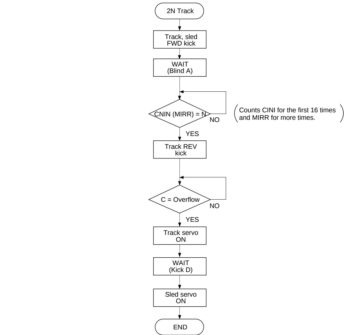
Fig. 3-11. (a) 2N-Track Jump Flow Chart
