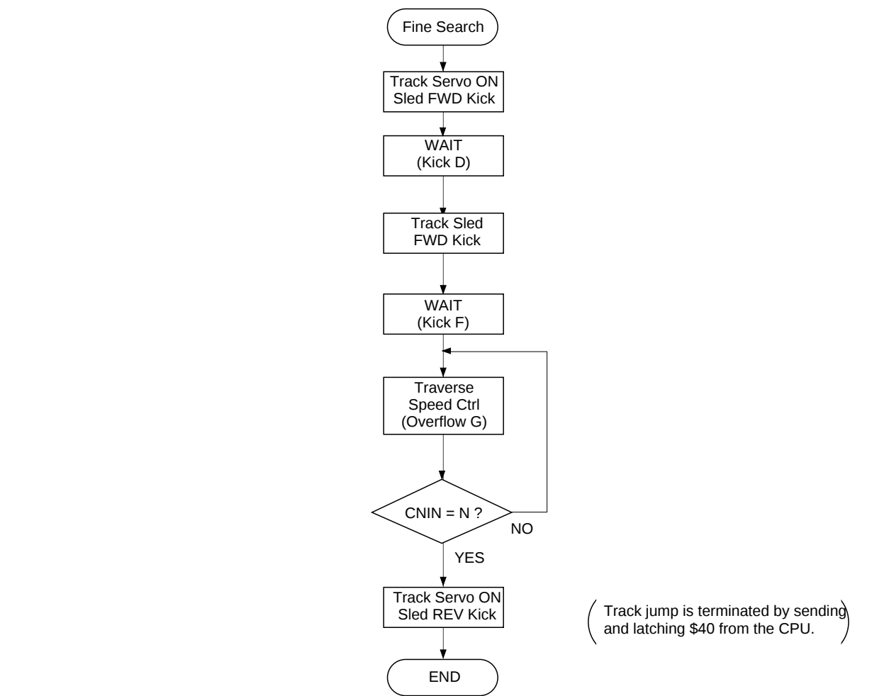
Fig. 3-12. (a) Fine Search Flow Chart
