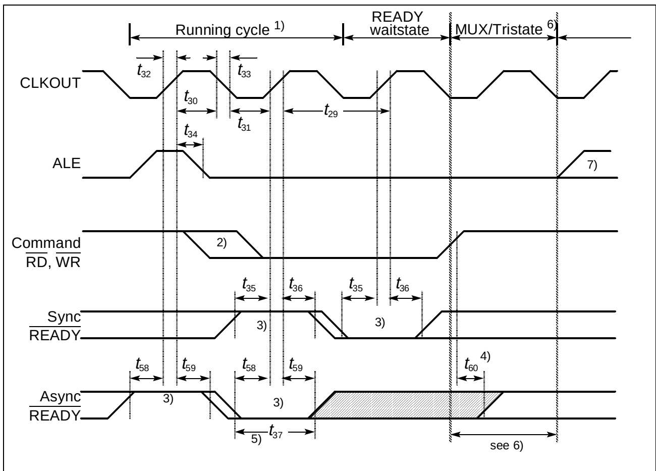
Figure 17 CLKOUT and READY
