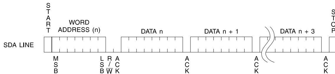
Figure 2. Page Write
