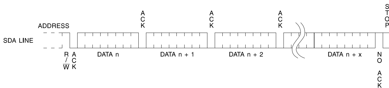
Figure 4. Sequential Read
