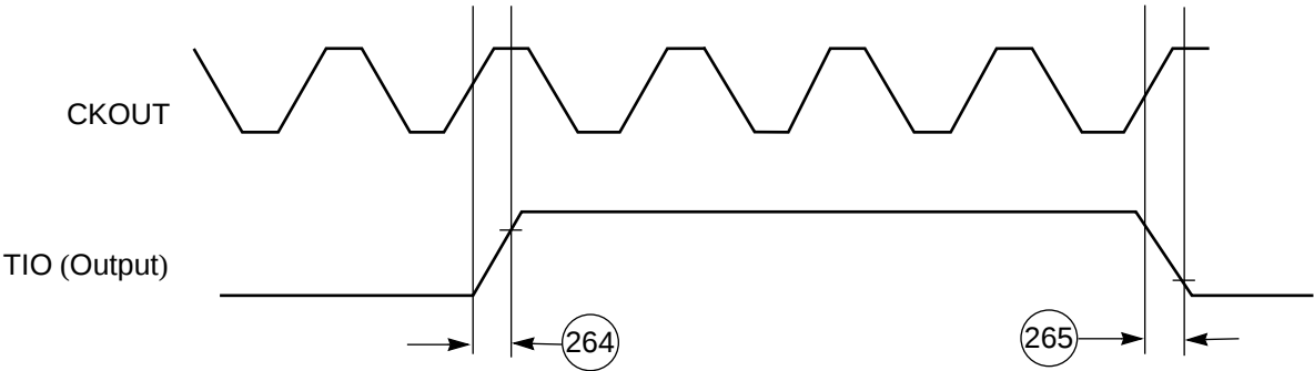
Figure 36 External Pulse Generation
