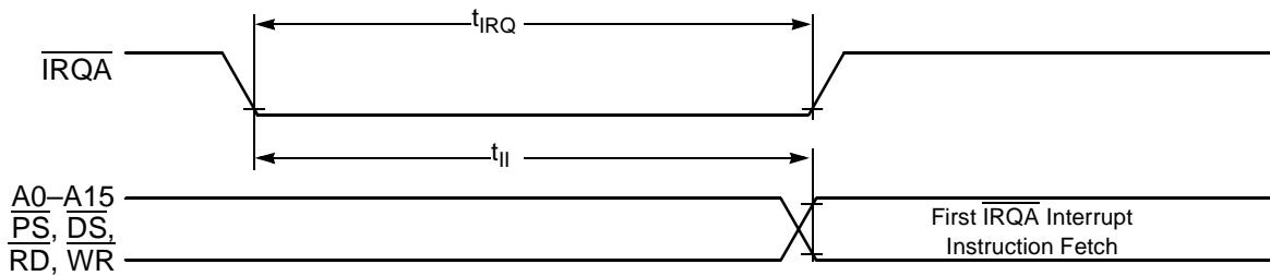
Figure 20. Recovery from Stop State Using \overline{\text{IRQA}} Interrupt Service
