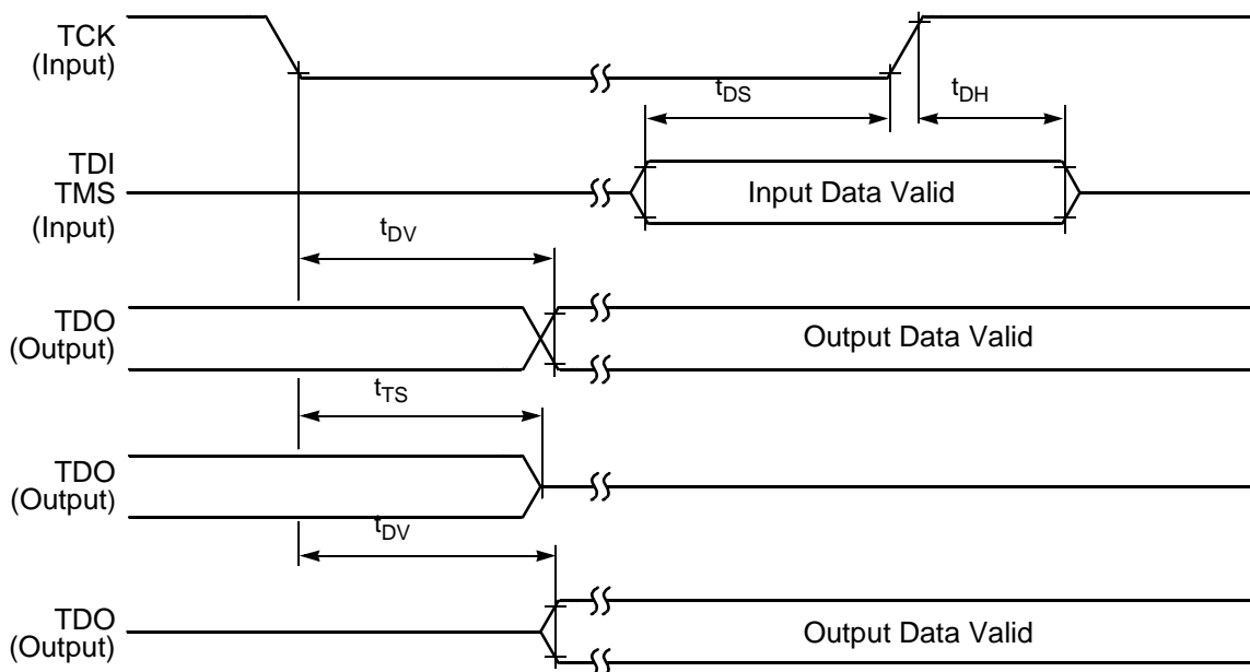
Figure 29. Test Clock Input Timing Diagram
