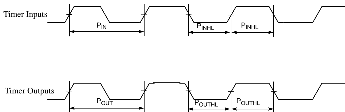
Figure 25. Timer Timing
