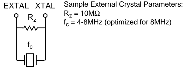
Figure 9. External Crystal Oscillator Circuit
