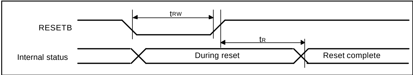
Figure 44. Reset Input Timing Diagram
