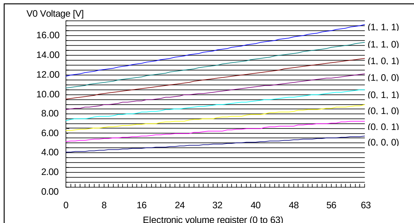
Figure 22. V0 Voltage by 1 + (R_b / R_a) and Electronic Volume Levels
