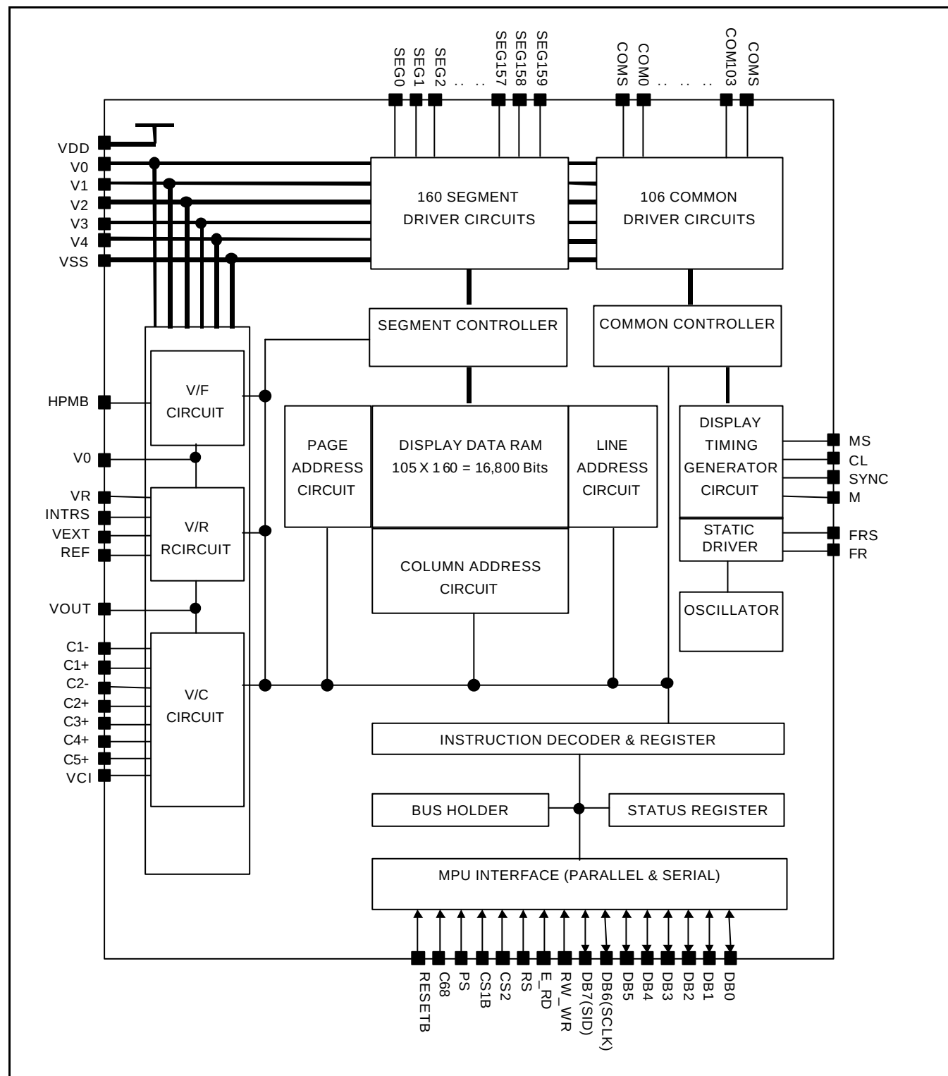
Figure 1. Block Diagram
