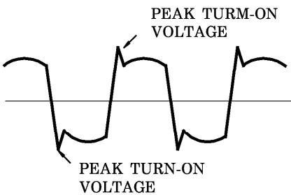
Fig.2 PEAK TURN-ON VOLTAGE WAVEFOM
