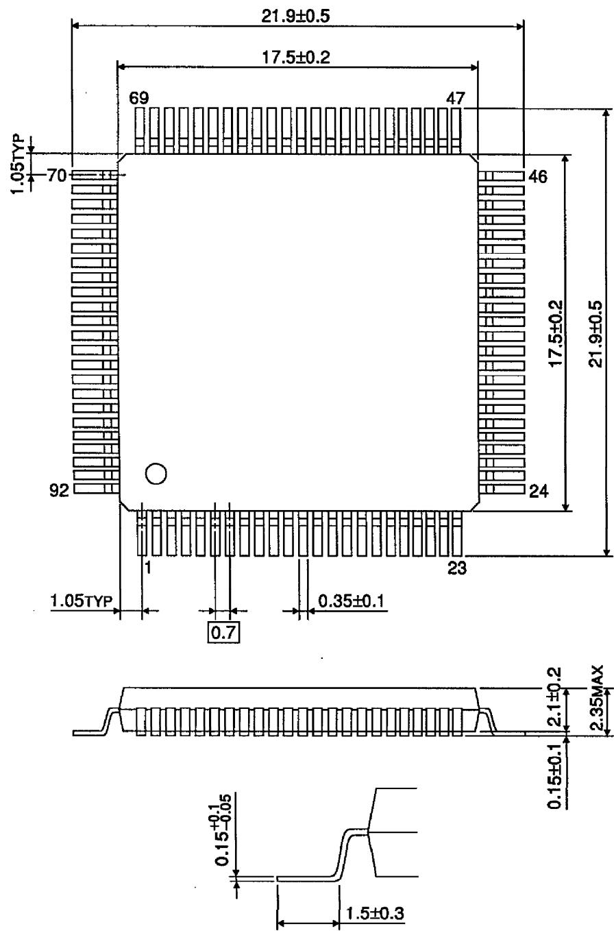
OUTLINE DRAWING QFP92-P-1818-0.70A
