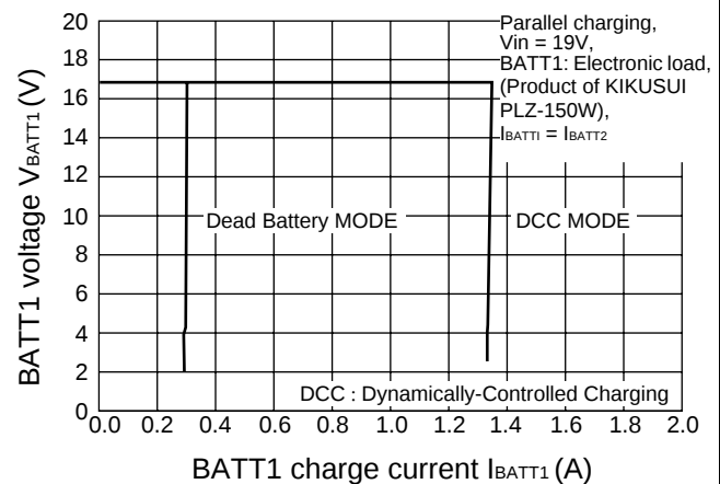
BATT voltage vs. BATT charge current
