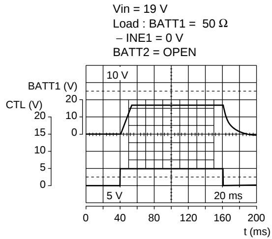
Soft start operating waveforms
