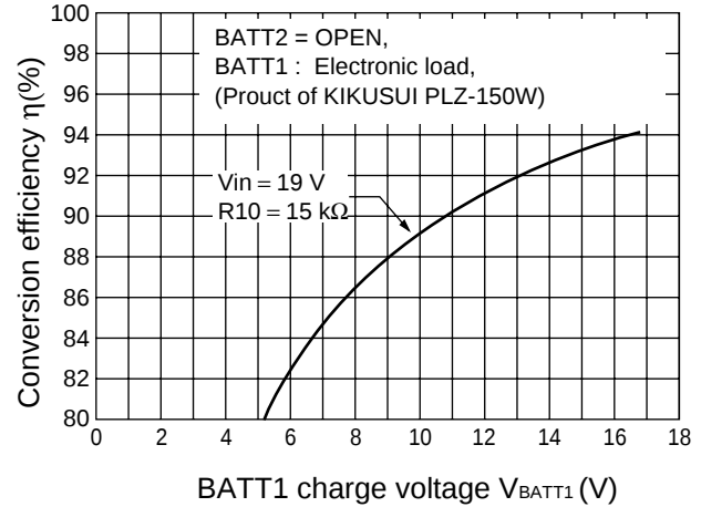
Conversion efficiency vs. charge voltage (Fixed current mode)
