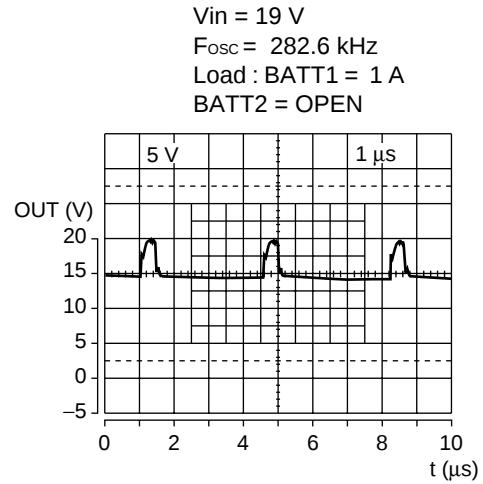
DC/DC converter switching waveforms
