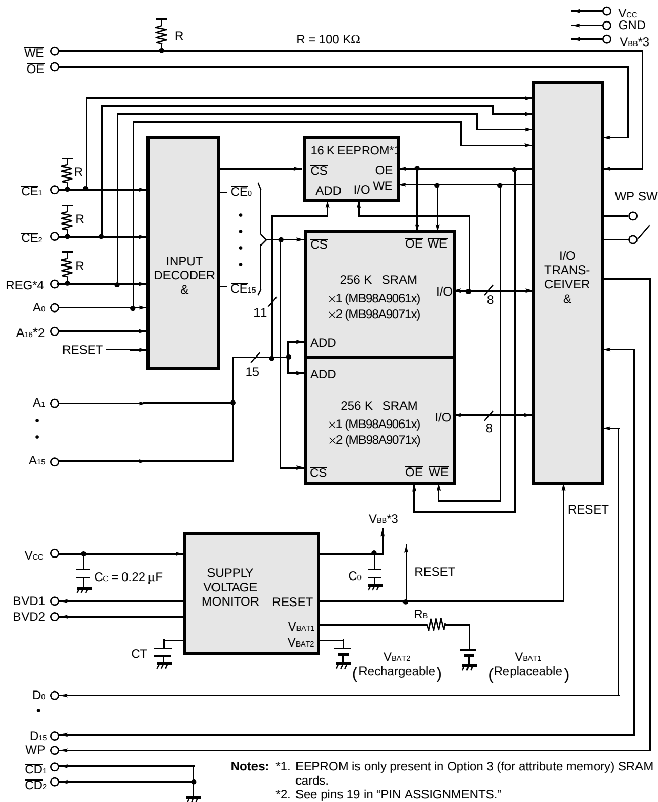
Fig. 1 - MB98A9061x/9071x BLOCK DIAGRAM
