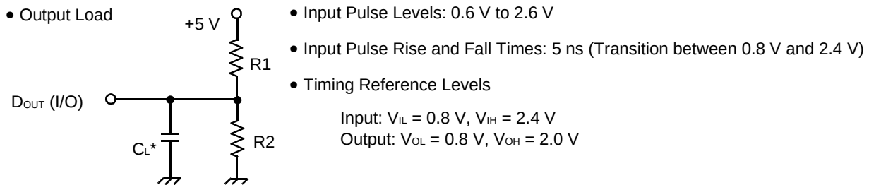
Fig. 3 – AC TEST CONDITIONS
