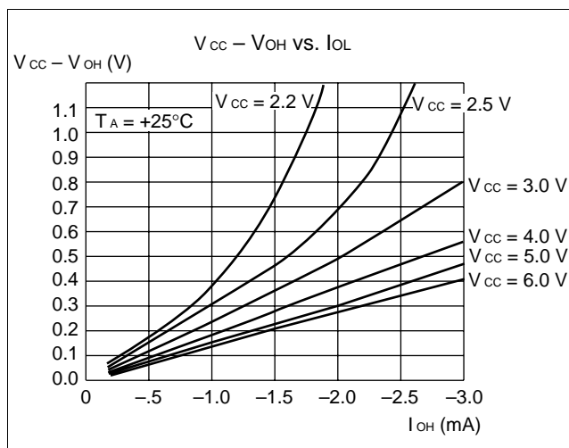
(2) “H” Level Output Voltage
