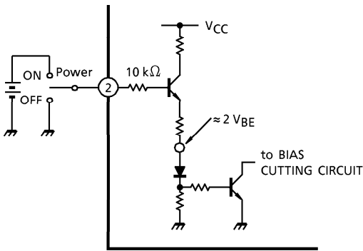
(Fig.2) With pin② set to High, Power is turned ON
