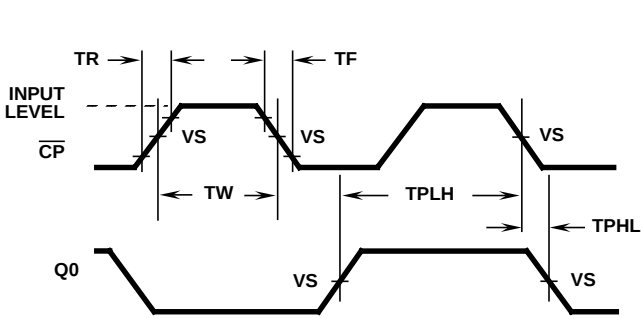
FIGURE 1. INPUT PULSE PRE-REQUISITE, PROPAGATION-DELAY, AND OUTPUT-TRANSITION TIMES
