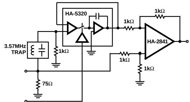
FIGURE 2. VIDEO DC RESTORER
