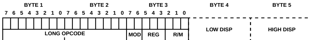
FIGURE 40B. LONG OPCODE FORMAT EXAMPLE
