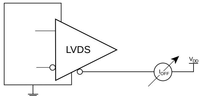
I_{OFF} SETUP
