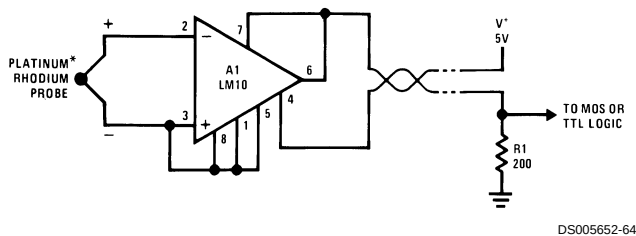
Flame Detector
