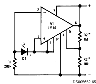
Light Level Sensor
