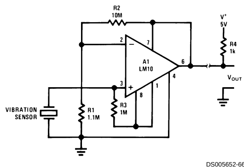
Remote Amplifier
