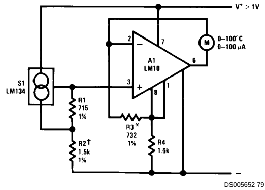
Thermometer
