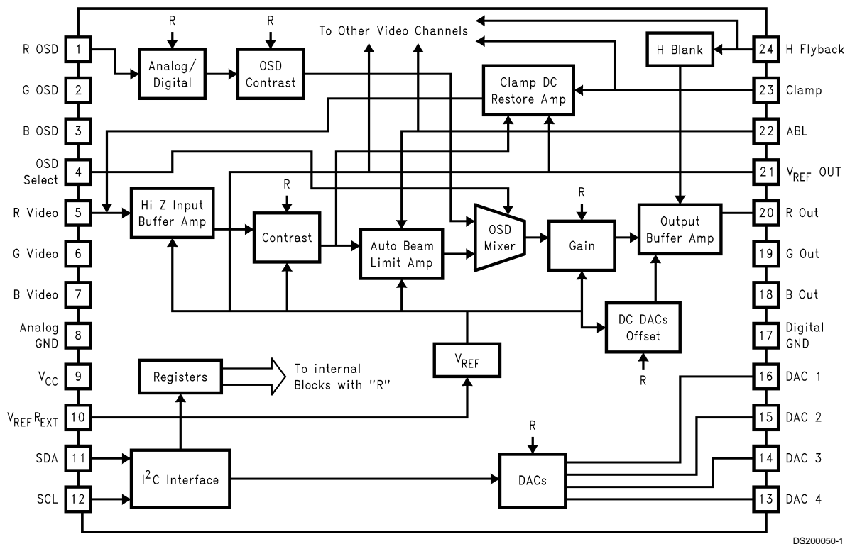
FIGURE 1. Order Number LM1267N See NS Package Number N24N
