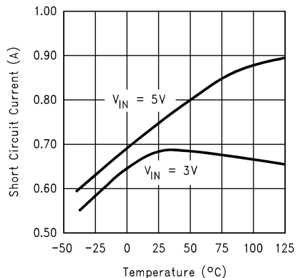
Short-Circuit Output Current vs Junction Temperature (Note 10)
