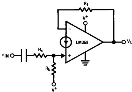
FIGURE 3. Biasing an Inverting AC Amplifier
