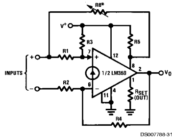
Difference Amplifier
