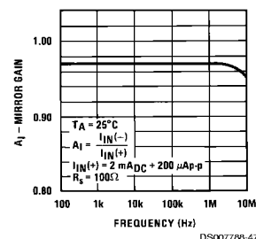
Mirror Gain
