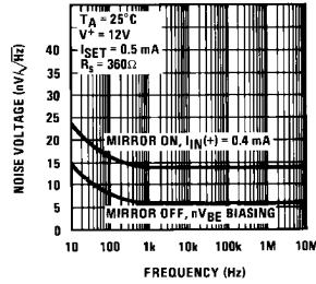
Noise Voltage
