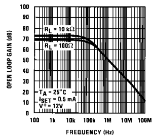
Open Loop Gain
