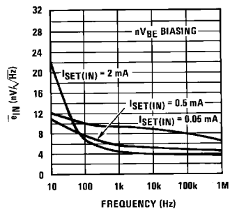
Typical Input Referred Noise Performance
