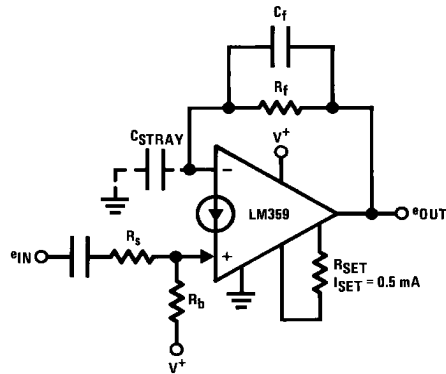
FIGURE 10. Best Method of Compensation
