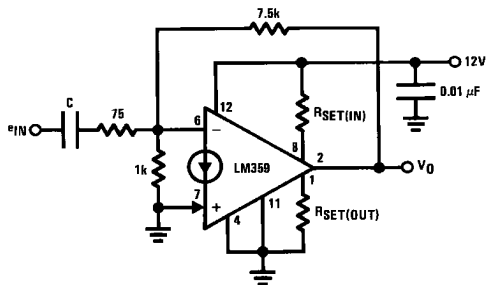
Noise Reduction using nV_{BE} Biasing
