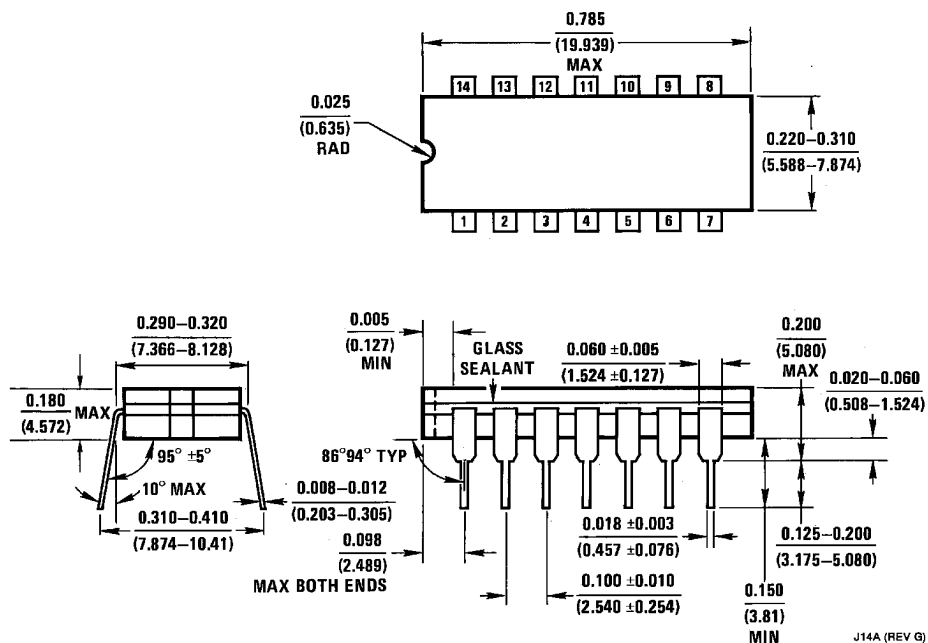
Ceramic Dual-In-Line Package (J) Order Number LM359J NS Package Number J14A
