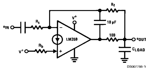
FIGURE 11. Isolating Large Capacitive Loads
