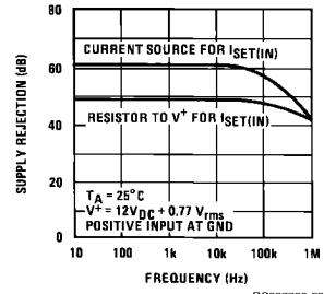
Supply Rejection
