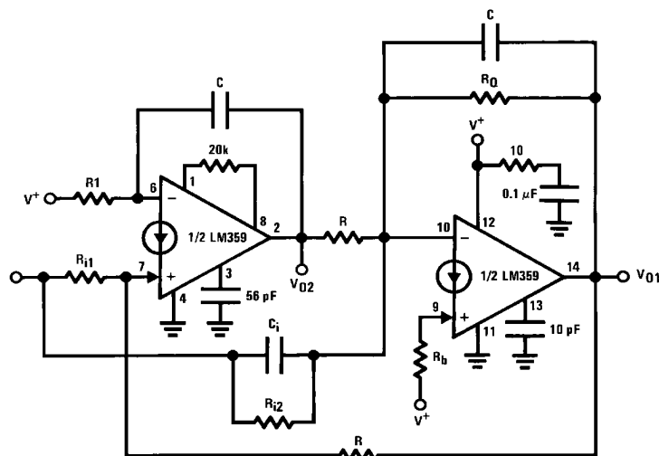
High Performance 2 Amplifier Biquad Filter(s)
