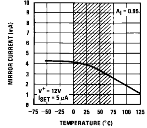
Mirror Current
