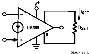
FIGURE 8. Single Resistor Programming of I_{SET}
