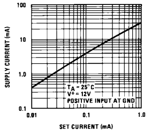
Supply Current
