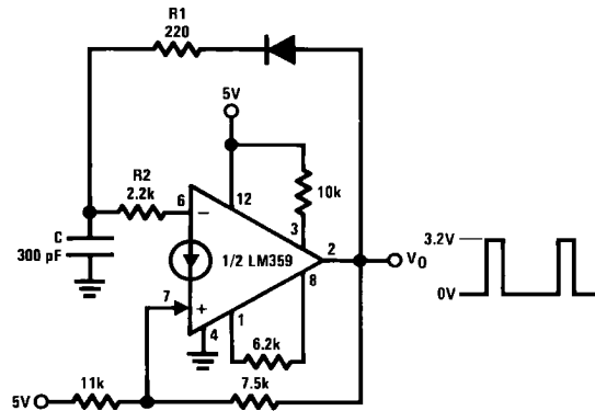
Pulse Generator
