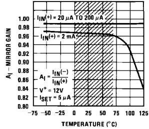
Mirror Gain
