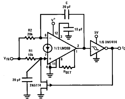
Voltage Controlled Oscillator
