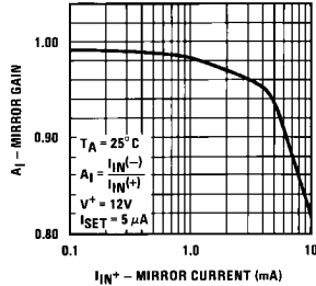
Mirror Gain
