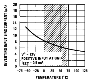
Inverting Input Bias Current
