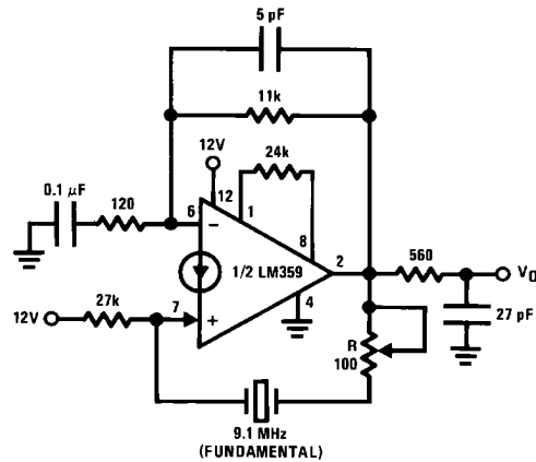
Crystal Controlled Sinewave Oscillator
