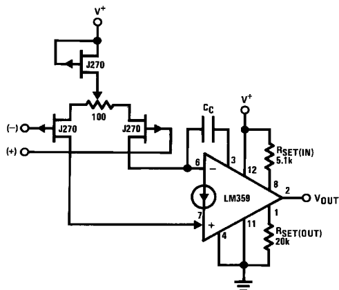
Adding a JFET Input Stage
