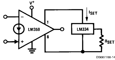
FIGURE 9. Current Source Programming of I_{SET}
