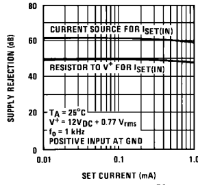
Supply Rejection
