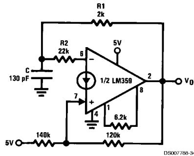
Squarewave Generator
