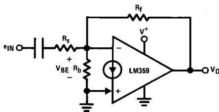
FIGURE 4. Biasing a Non-Inverting AC Amplifier
