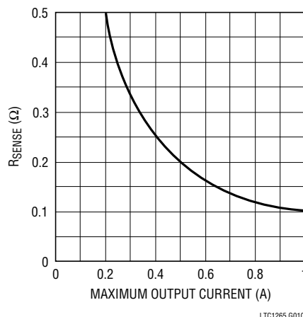
Figure 2. Selecting R_{\text{SENSE}}
