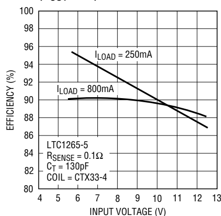
Efficiency vs Input Voltage (V_{\text{OUT}} = 5\text{V})
