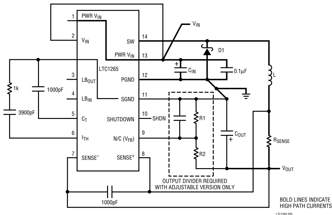
Figure 5. LTC1265 Layout Diagram (See Board Layout Checklist)
