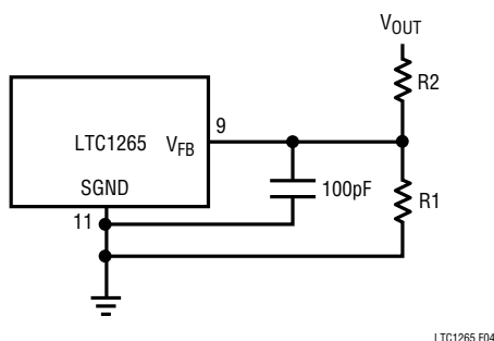
Figure 4. LTC1265 Adjustable Configuration
