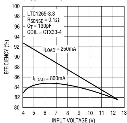
Efficiency vs Input Voltage (V_{\text{OUT}} = 3.3\text{V})
