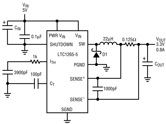
Figure 8. Design Example Circuit
