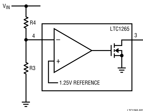
Figure 3. Low-Battery Comparator
