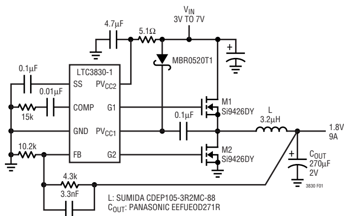
Figure 1. High Efficiency 3.3V to 1.8V Power Converter
