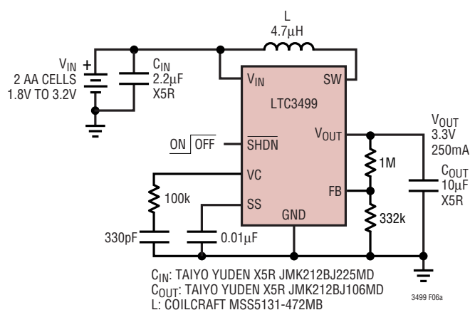
Two Cells to 3.3V, 250mA
