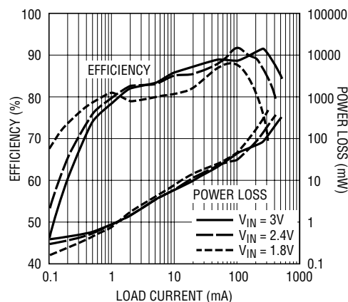
Two Cells to 3.3V Efficiency
