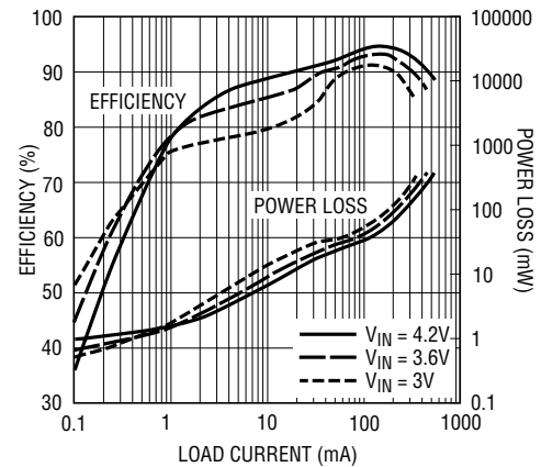
Lithium-Ion to 5V Efficiency
