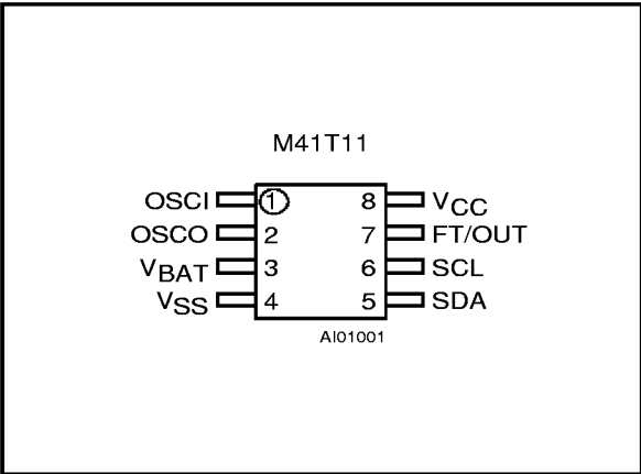
Figure 2. SOIC Pin Connections
