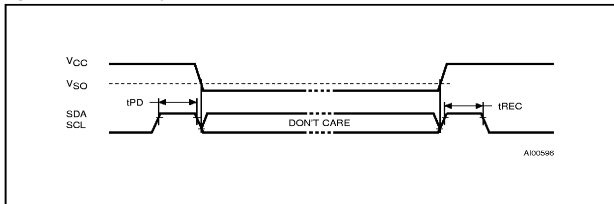
Figure 5. Power Down/Up Mode AC Waveforms
