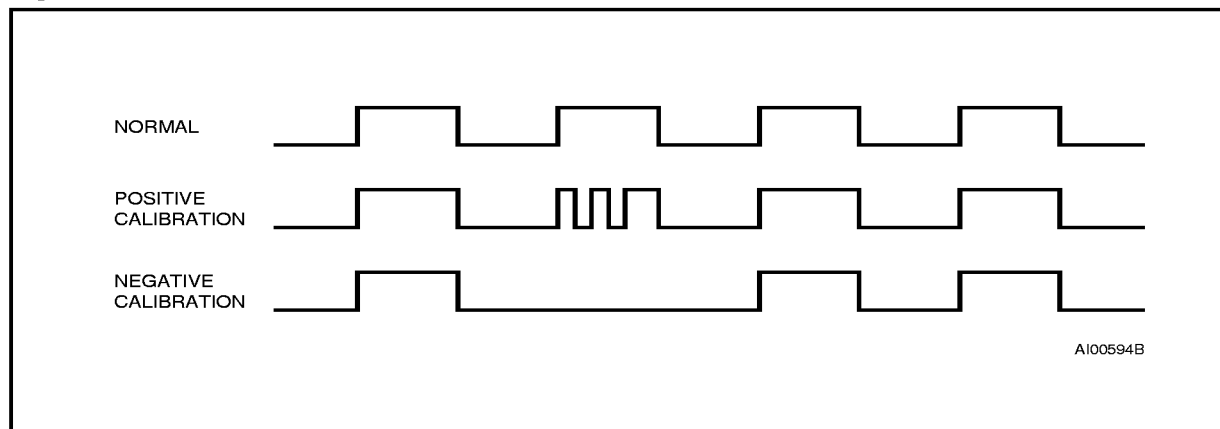
Figure 13. Clock Calibration
