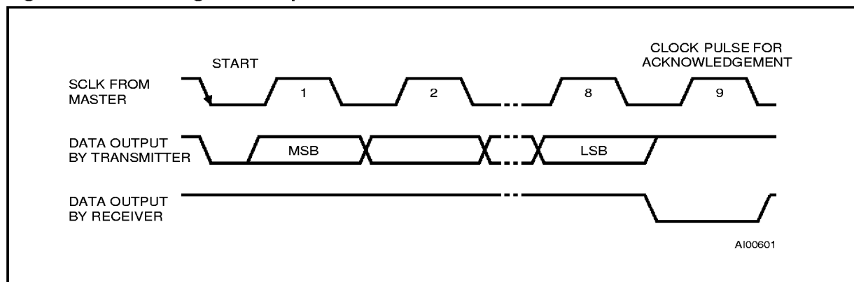
Figure 7. Acknowledgement Sequence
