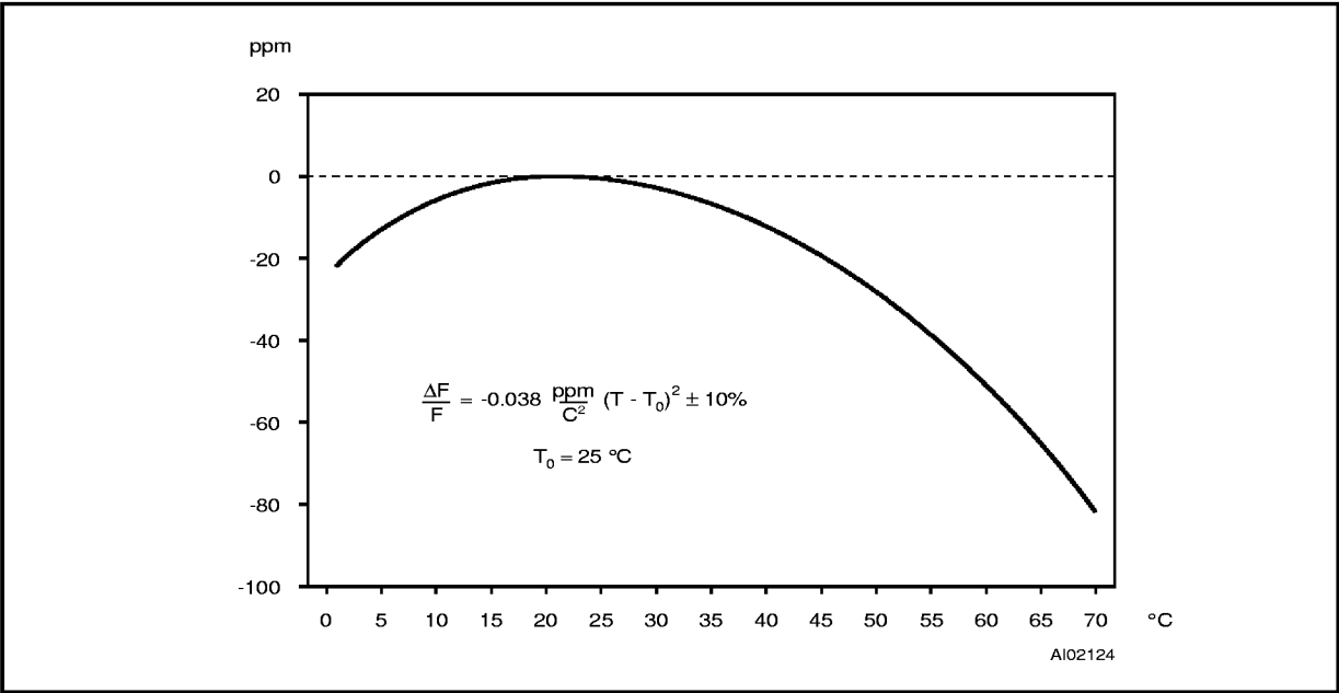
Figure 14. Crystal Accuracy Across Temperature
